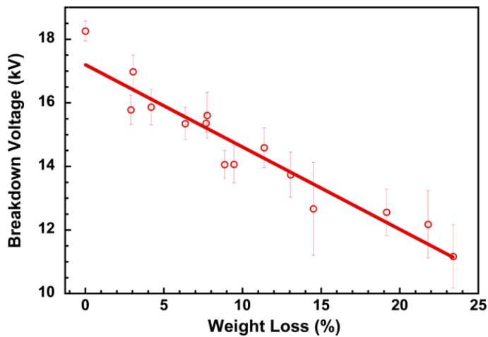
Figure 5: Measured breakdown voltage of degraded Kapton film (symbols) with best linear fit (solid line).
