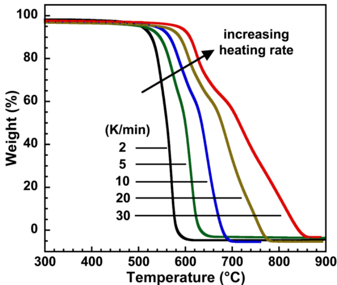
Figure 2: TG curves for Kapton in an oxidative environment.
