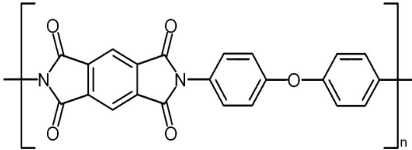
Figure 1: Chemical structure of Kapton.
