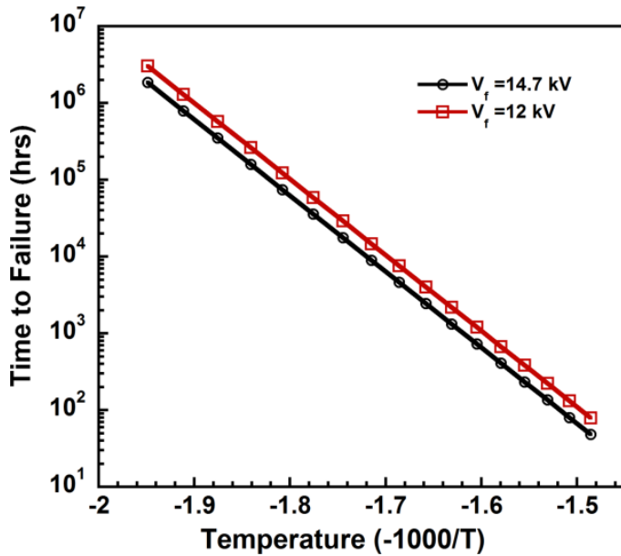
Figure 6: Predicted time to failure at 12 and 14.7 kV and for isothermal temperatures ranging from 250 to 400°C.
