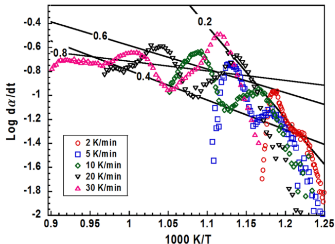
Figure 3: Friedman plot from the data shown in Figure 2. Four isoconversional fractional weight loss trend lines are represented for 0.2, 0.4, 0.6, and 0.8 fractional weight loss.
