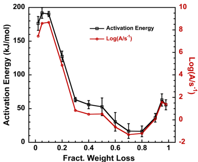
Figure 4: Kinetic parameters obtained by Friedman analysis of TG analysis data on Kapton.
